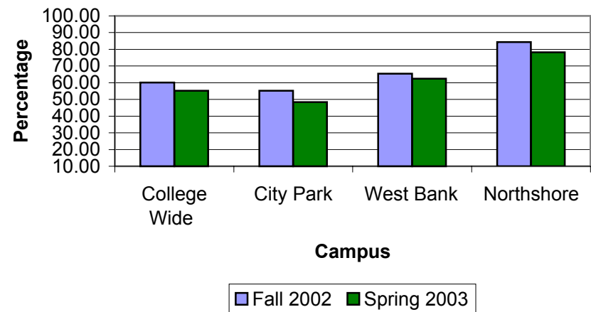
English 062 Remediation Completion Rate
