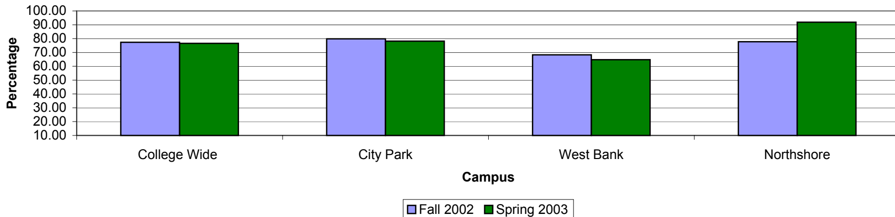
Math 096 Success Rate
