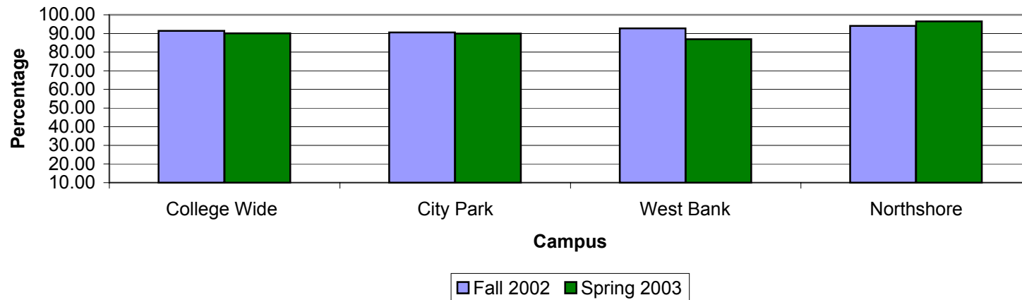
English 062 Success Rate
