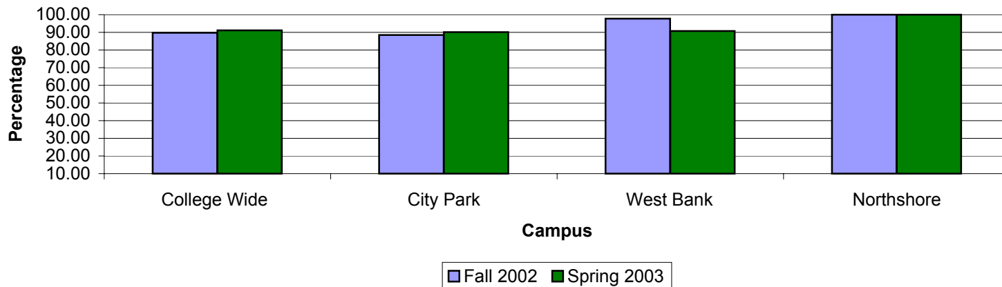
English 061 Success Rate
