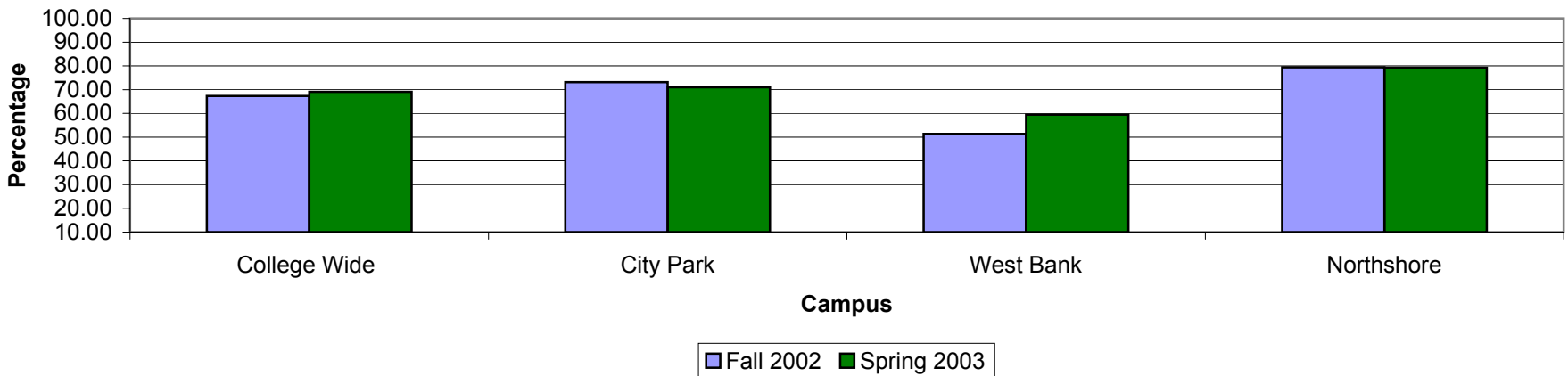
Math 095 Success Rate
