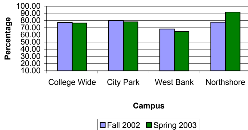
Math 096 Remediation Rate
