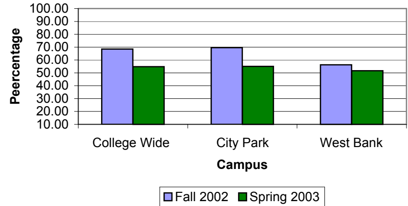
English 063 Remediation Completion Rate
