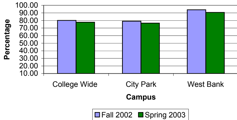
English 063 Retention Rate
