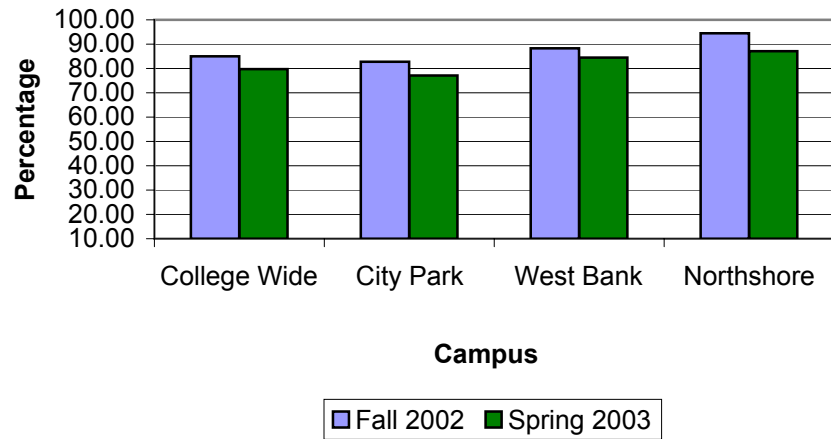
English 062 Retention Rate
