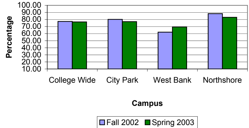
Math 091 Remediation Rate
