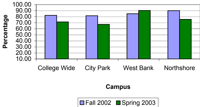
English 061 Retention Rate
