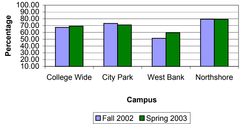
Math 095 Remediation Rate
