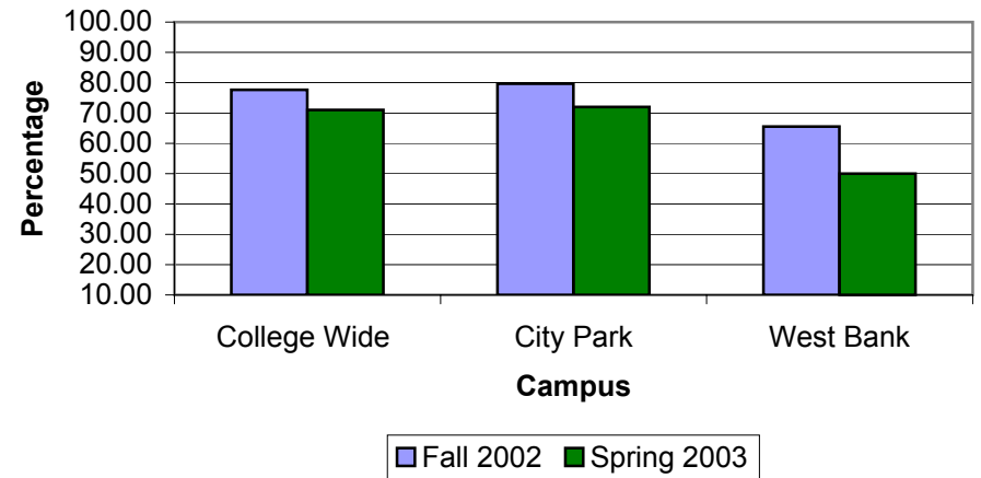
Math 090 Remediation Rate
