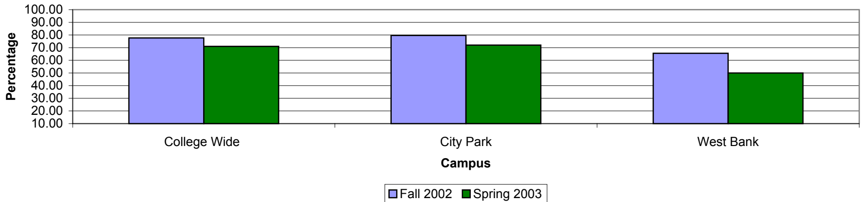
Math 090 Success Rate
