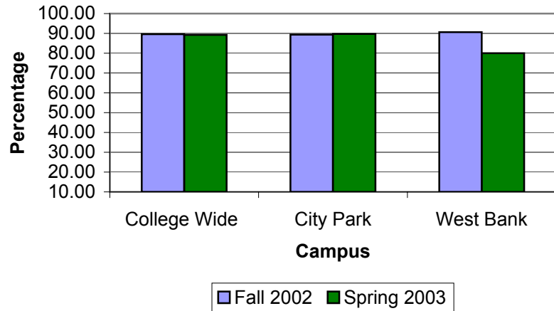
Math 090 Retention Rate
