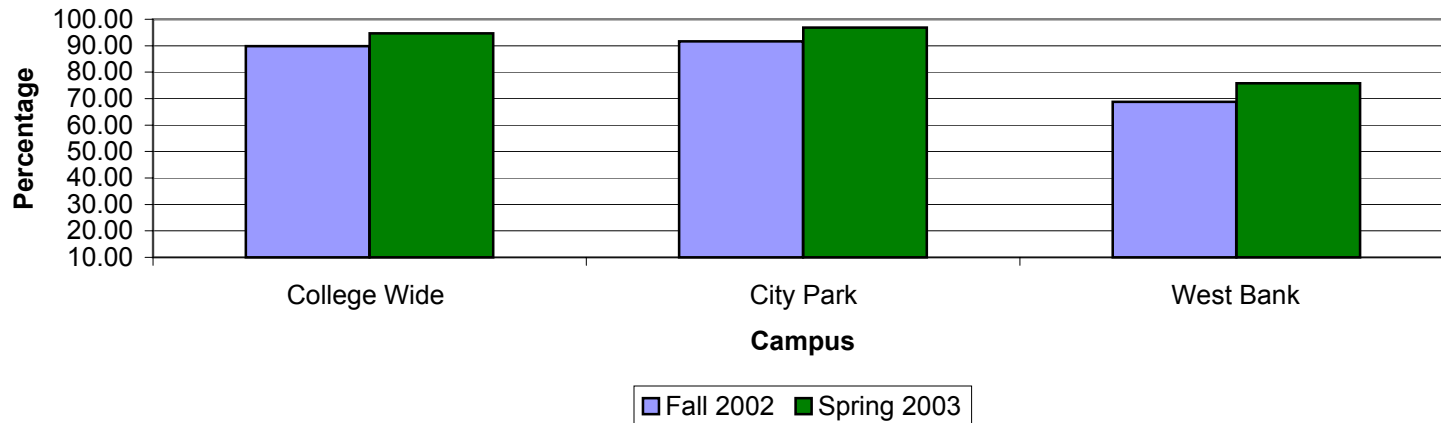
English 063 Success Rate
