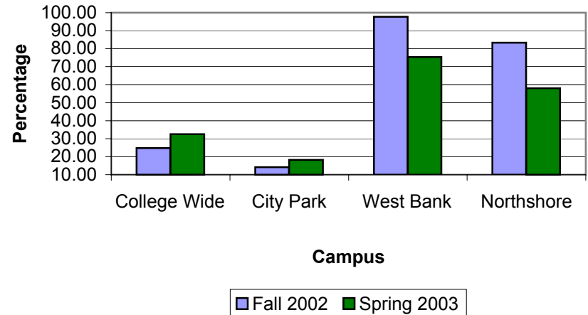
English 061 Remediation Completion Rate
