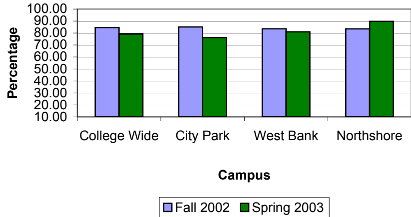
Math 091 Retention Rate
