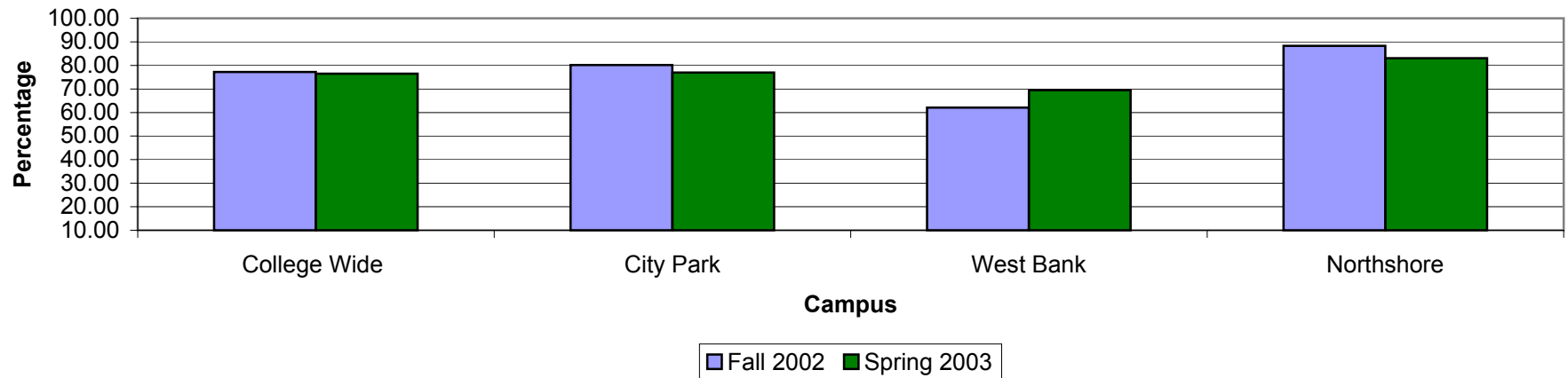
Math 091 Success Rate
