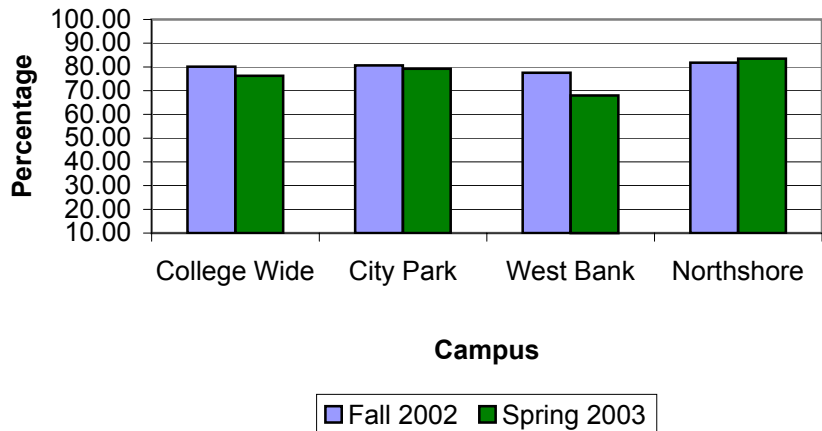
Math 096 Retention Rate
