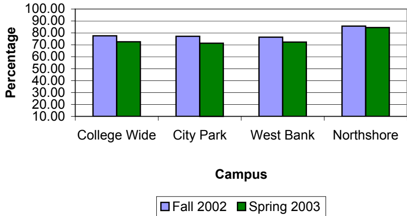
Math 095 Retention Rate
